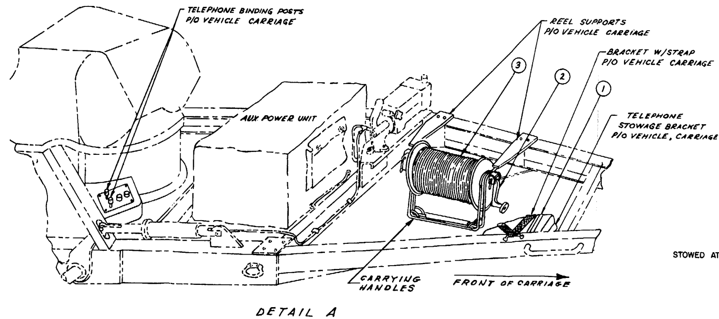
Figure 2-1. Telephone sets and reel equipment installed in Gun, AAA, 20mm, XM167.
